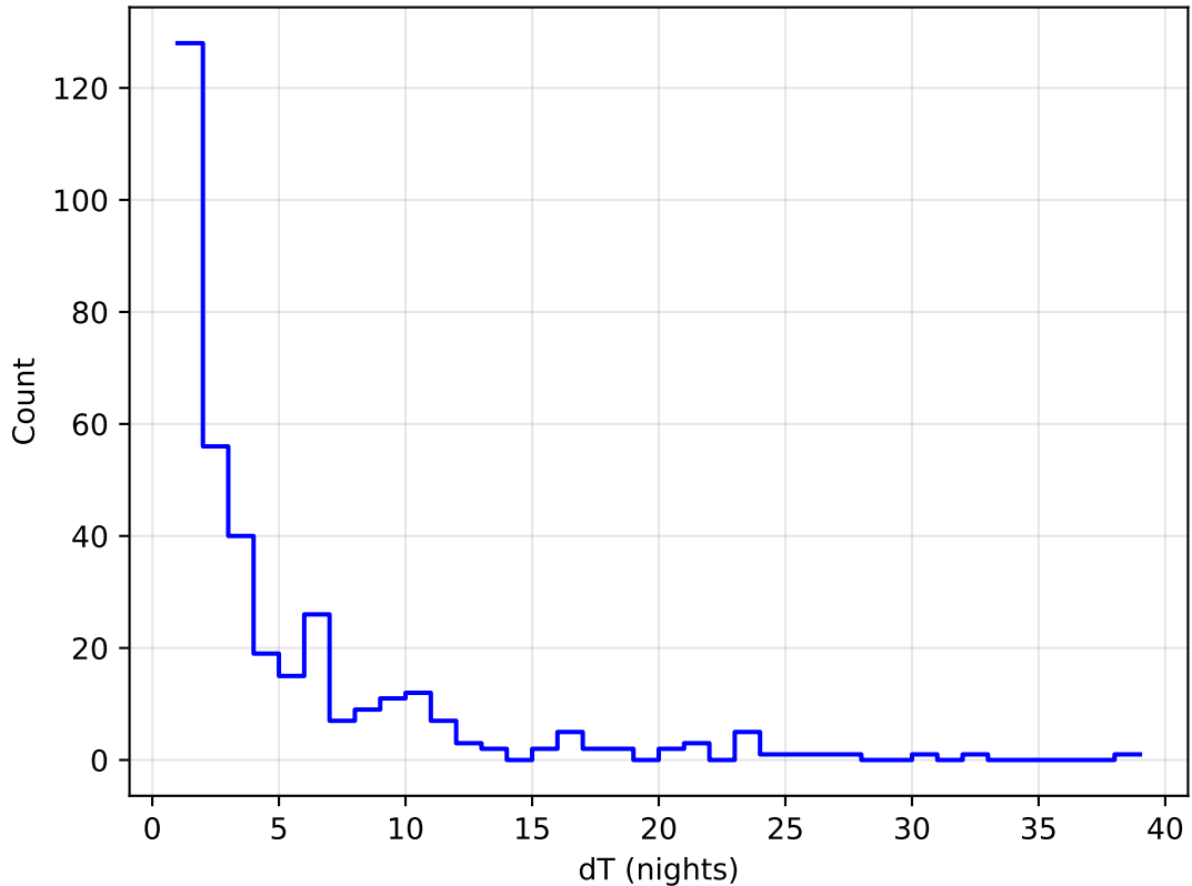
roll_pause_mjdp180_v3.4_10yrs all bands: DD:WFD Delta Nights Histogram
