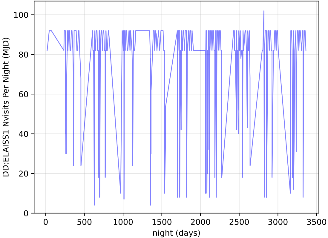
roll_pause_mjdp180_v3.4_10yrs all bands: DD:ELAISS1 Nvisits Per Night
