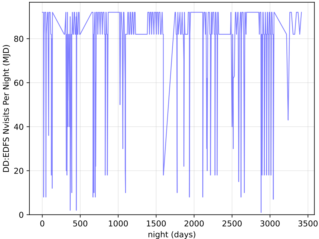
roll_pause_mjdp180_v3.4_10yrs all bands: DD:EDFS Nvisits Per Night
