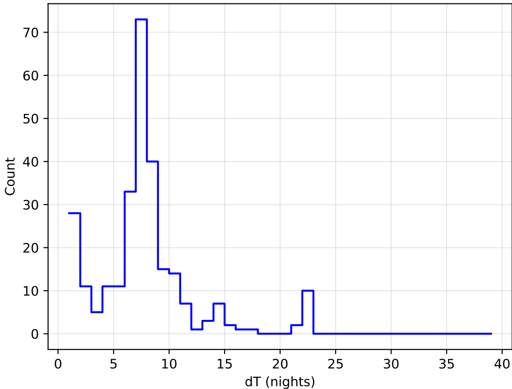
roll_pause_mjdp180_v3.4_10yrs all bands: DD:EDFS Delta Nights Histogram
