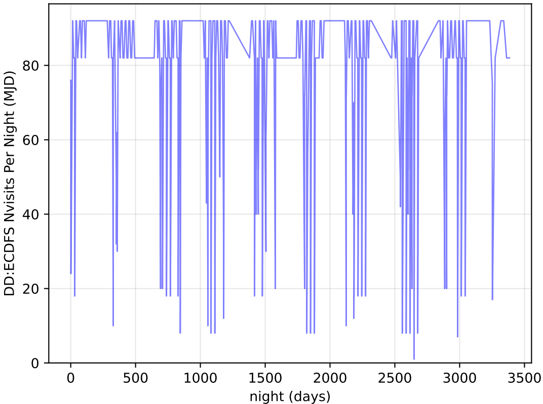
roll_pause_mjdp180_v3.4_10yrs all bands: DD:ECDFS Nvisits Per Night
