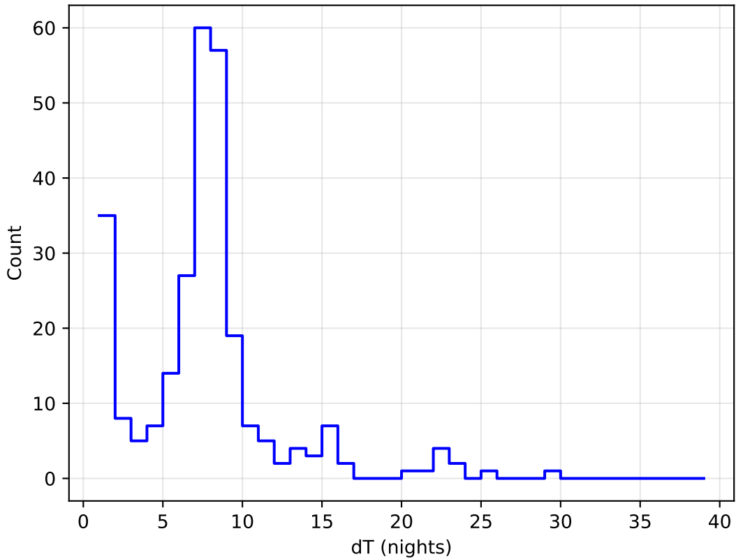
roll_pause_mjdp180_v3.4_10yrs all bands: DD:ECDFS Delta Nights Histogram
