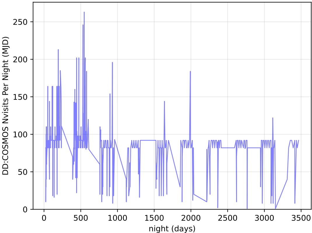
roll_pause_mjdp180_v3.4_10yrs all bands: DD: COSMOS Nvisits Per Night
