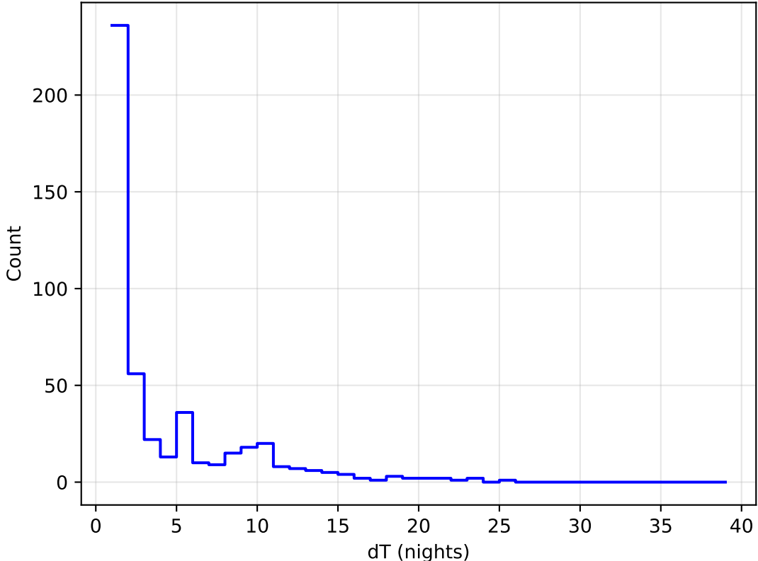
roll_pause_mjdp180_v3.4_10yrs all bands: DD: COSMOS Delta Nights Histogram
