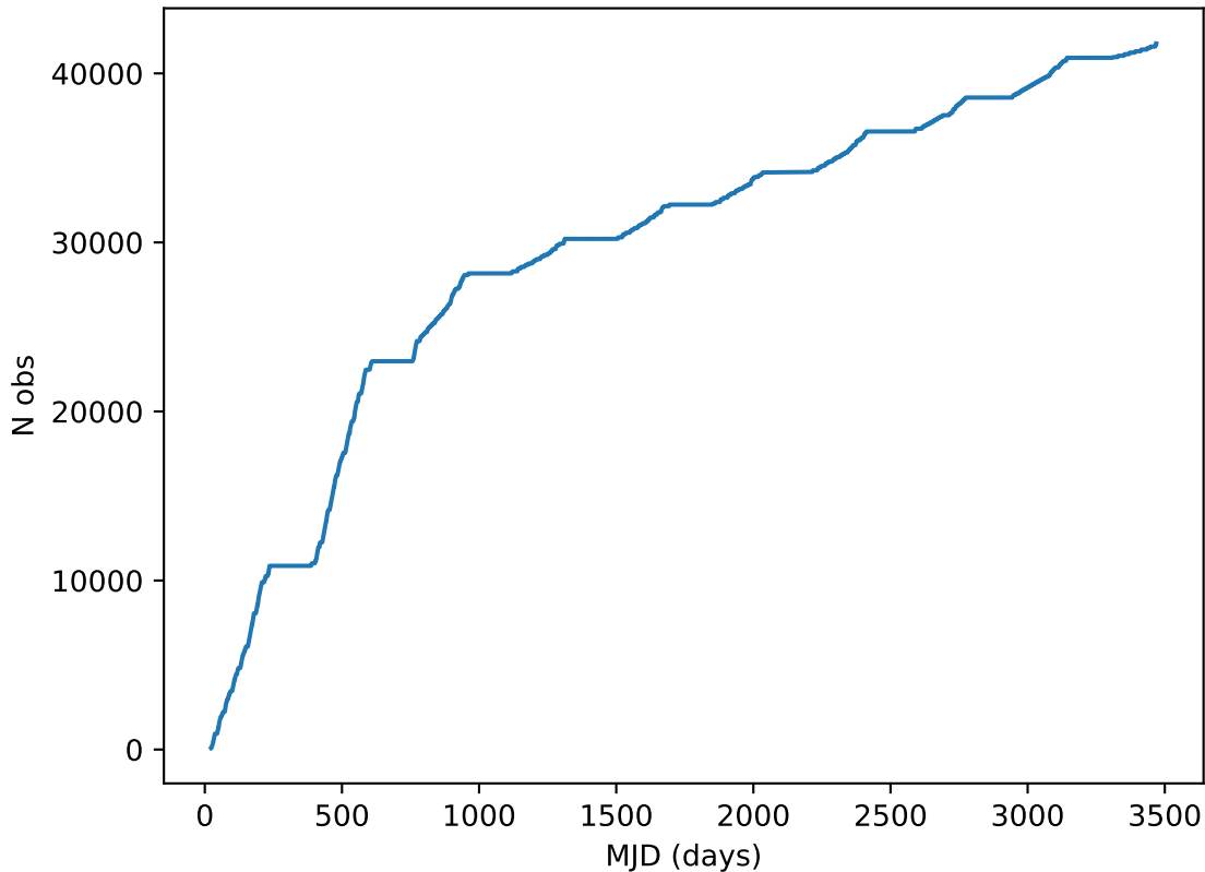
roll_pause_mjdp180_v3.4_10yrs all bands: DD: COSMOS Cumulative NVisits
