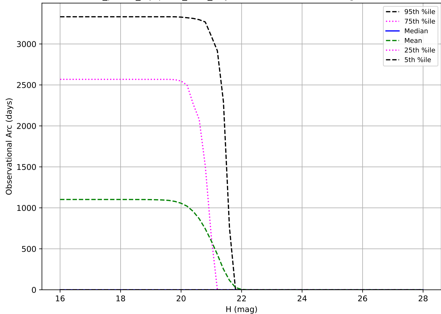
roll_pause_mjdp120_v3.4_10yrs: Observational Arc Length Vatira
