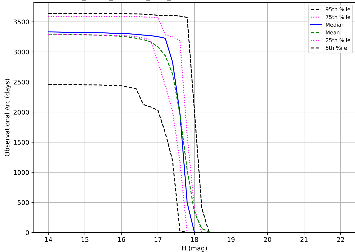
roll_pause_mjdp120_v3.4_10yrs: Observational Arc Length Trojan
