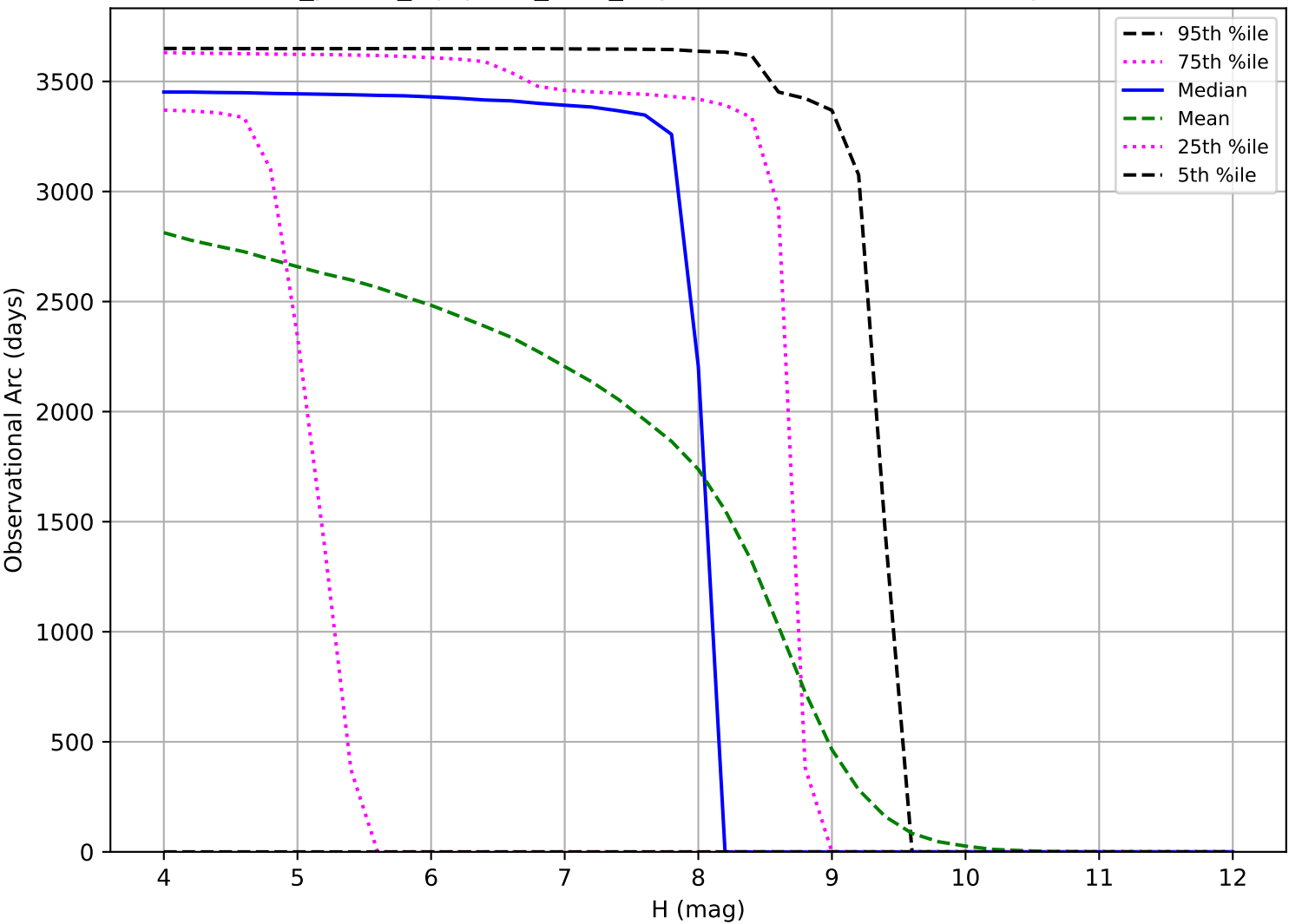
roll_pause_mjdp120_v3.4_10yrs: Observational Arc Length TNO
