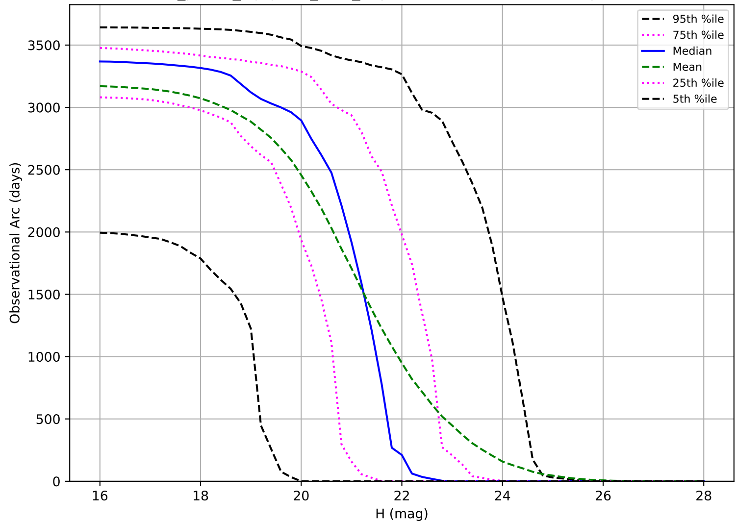
roll_pause_mjdp120_v3.4_10yrs: Observational Arc Length PHA
