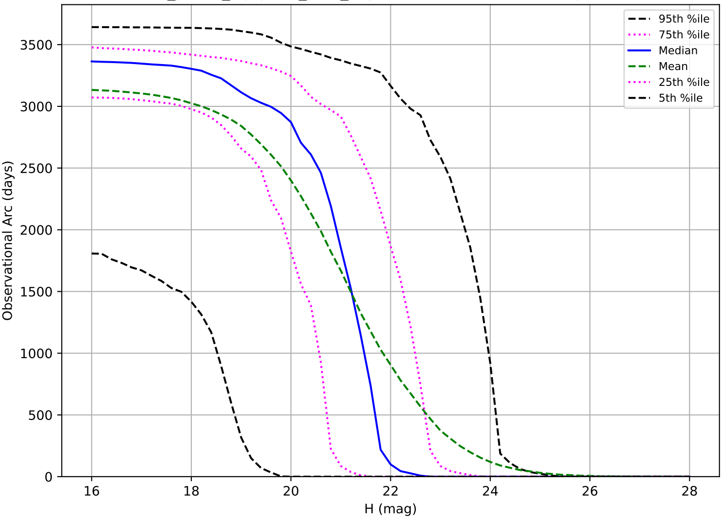
roll_pause_mjdp120_v3.4_10yrs: Observational Arc Length NEO
