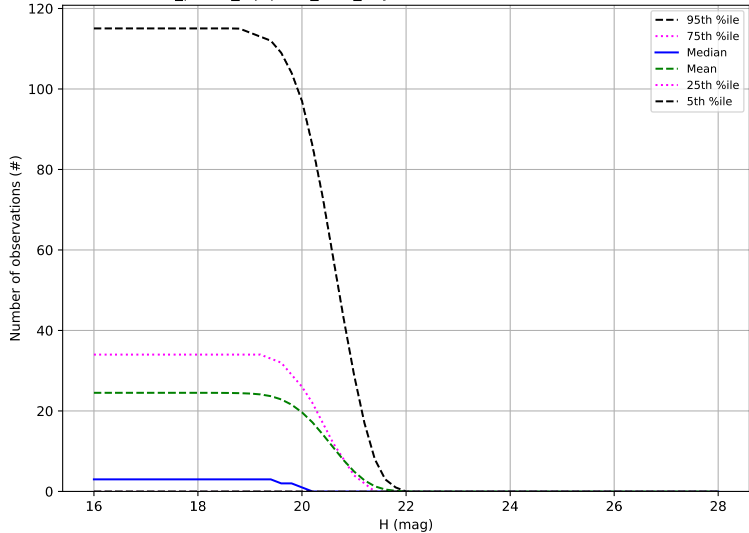
roll_pause_mjdp120_v3.4_10yrs: Number of observations Vatira
