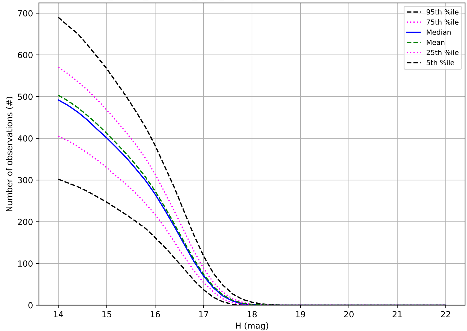
roll_pause_mjdp120_v3.4_10yrs: Number of observations Trojan
