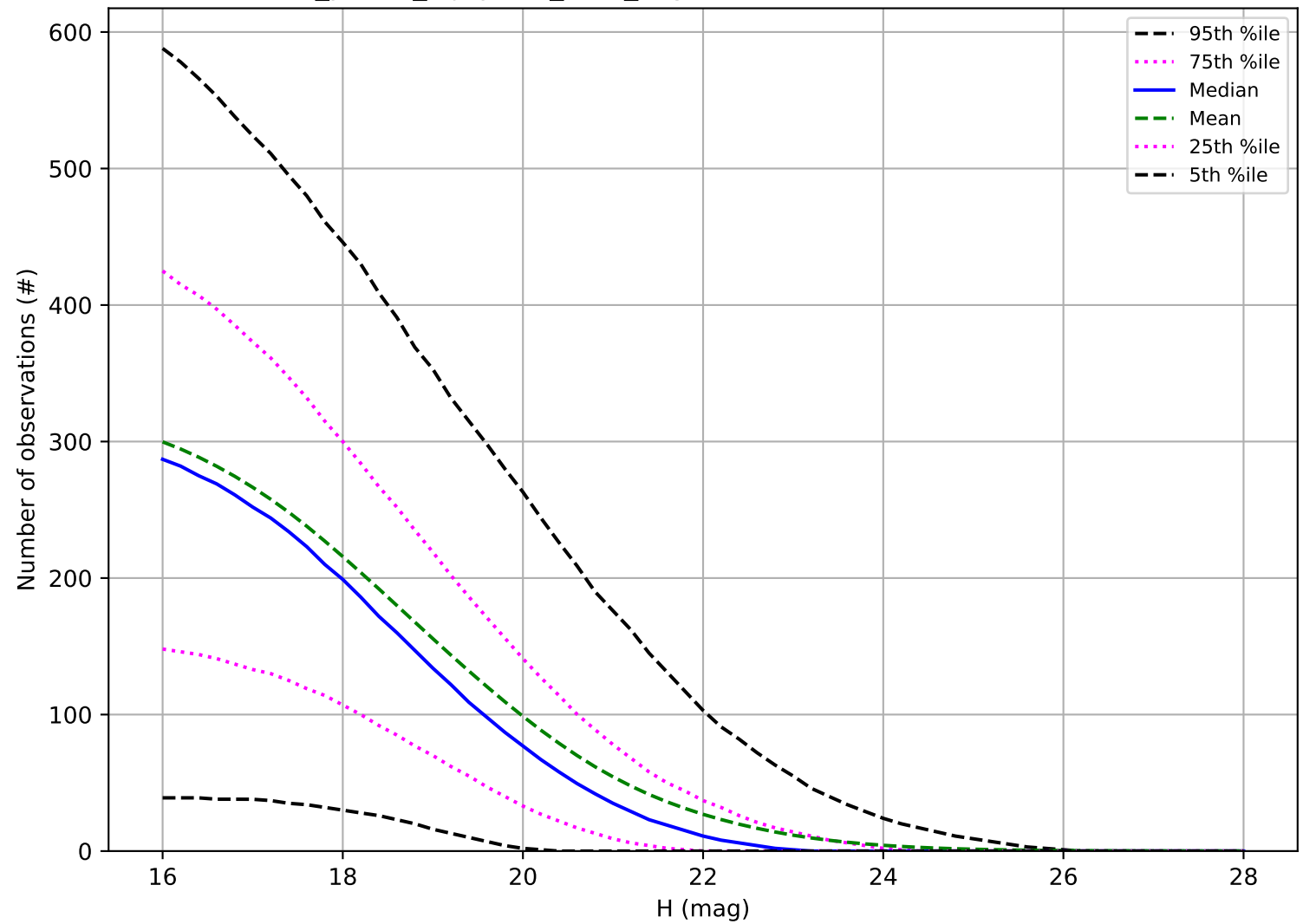
roll_pause_mjdp120_v3.4_10yrs: Number of observations PHA
