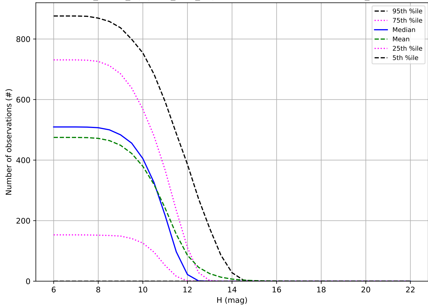
roll_pause_mjdp120_v3.4_10yrs: Number of observations OCC_r20
