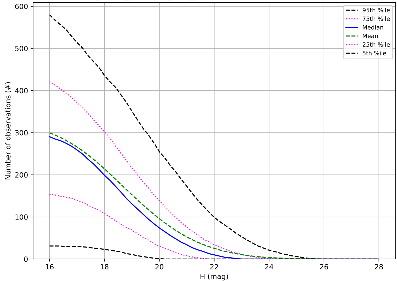
roll_pause_mjdp120_v3.4_10yrs: Number of observations NEO
