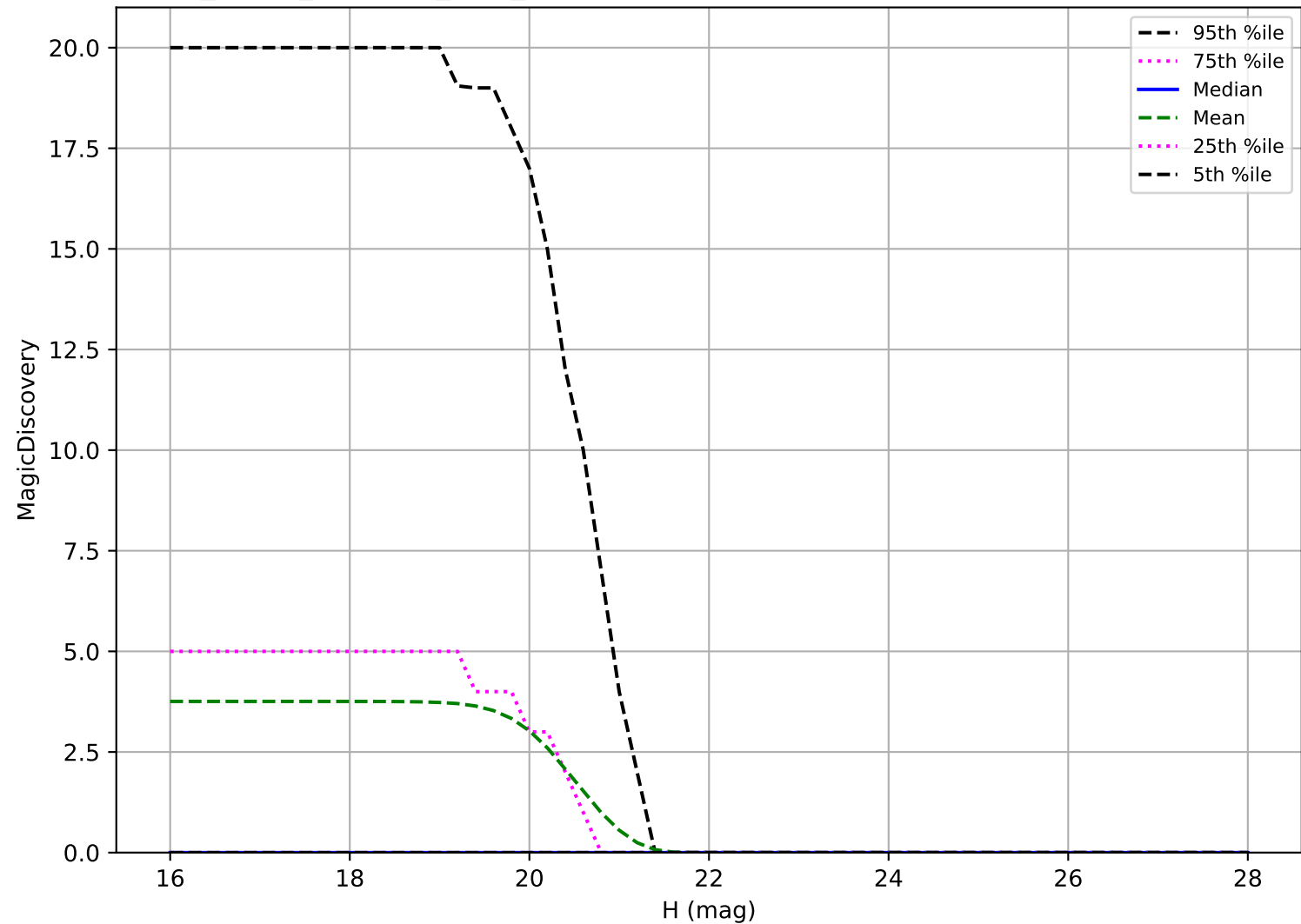
roll_pause_mjdp120_v3.4_10yrs: Vatira 6 detections in 60 nights detection loss
