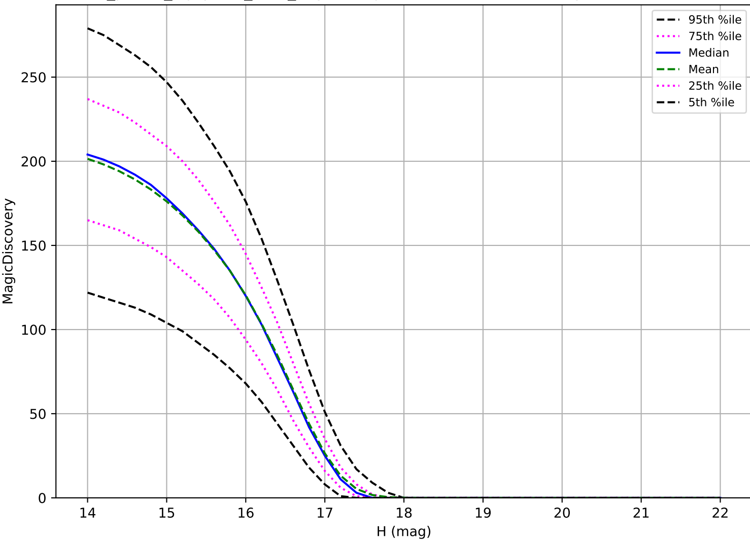
roll_pause_mjdp120_v3.4_10yrs: Trojan 6 detections in 60 nights detection loss
