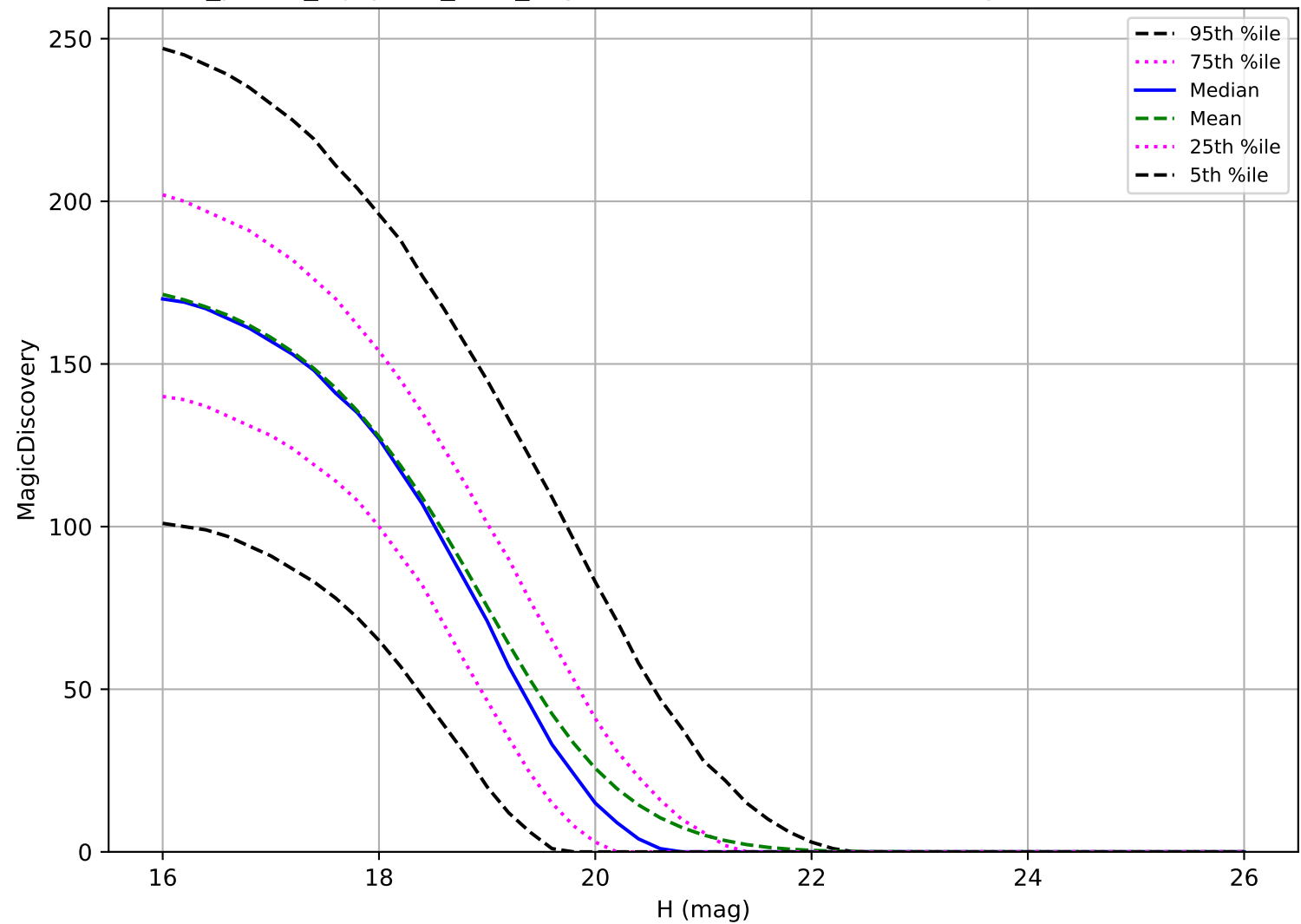
roll_pause_mjdp120_v3.4_10yrs: MBA 6 detections in 60 nights detection loss
