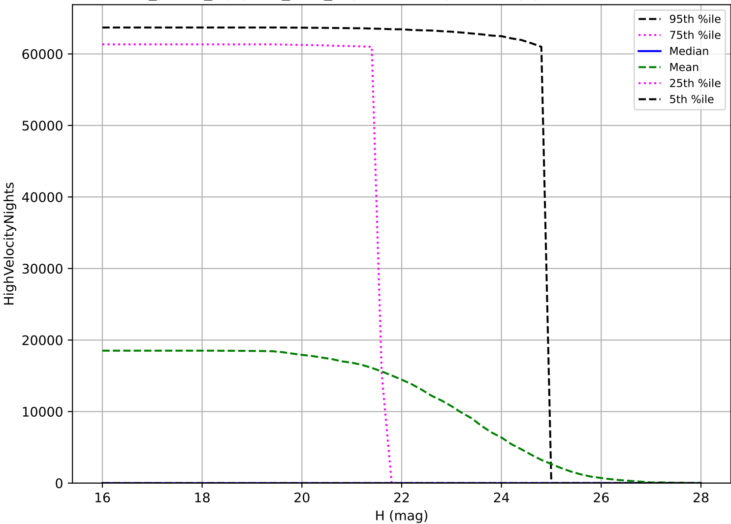
roll_pause_mjdp120_v3.4_10yrs: NEO High velocity pair detection loss
