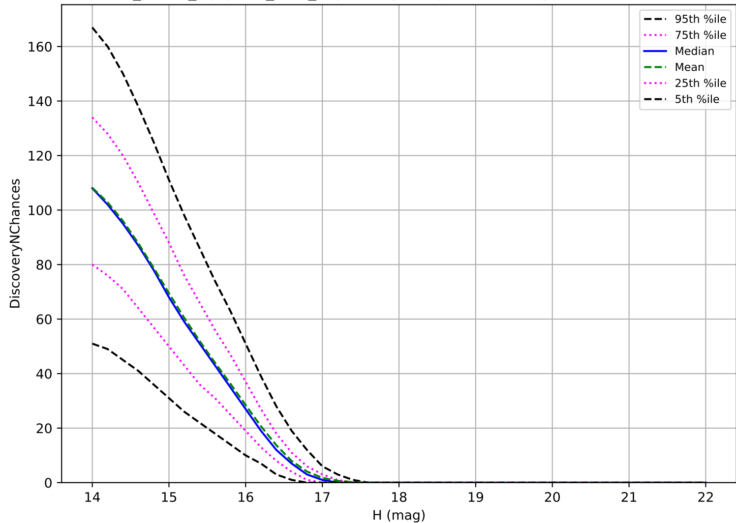
roll_pause_mjdp120_v3.4_10yrs: Trojan 3 pairs in 15 nights detection loss
