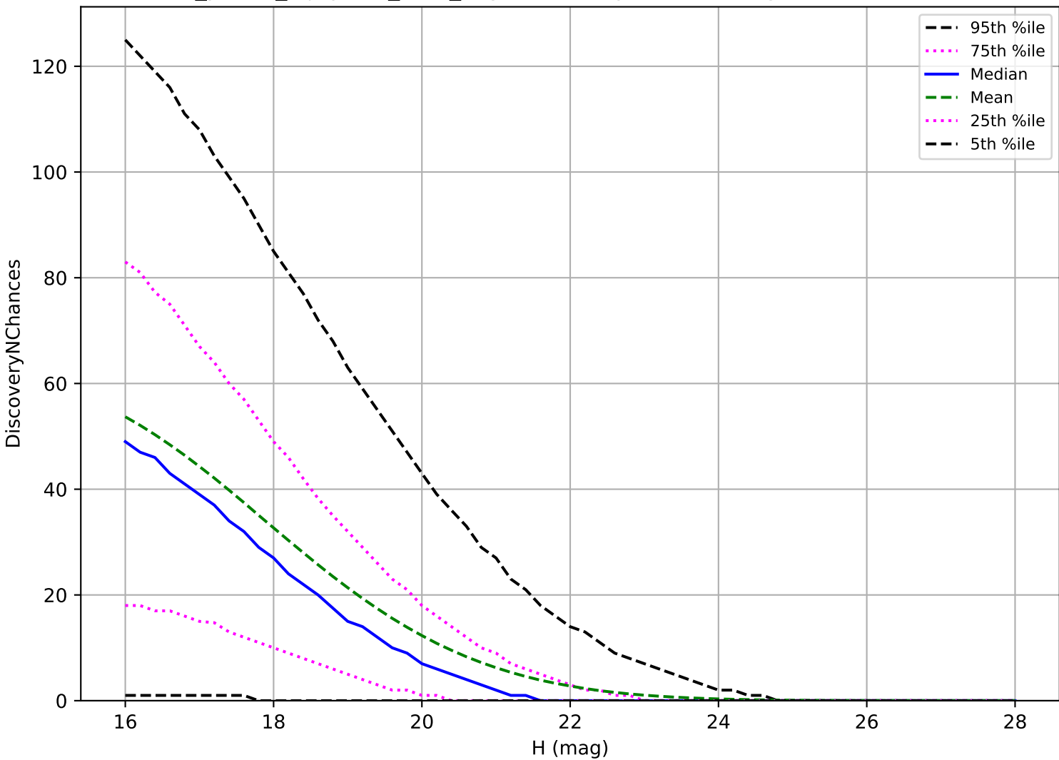
roll_pause_mjdp120_v3.4_10yrs: PHA 3 pairs in 15 nights detection loss
