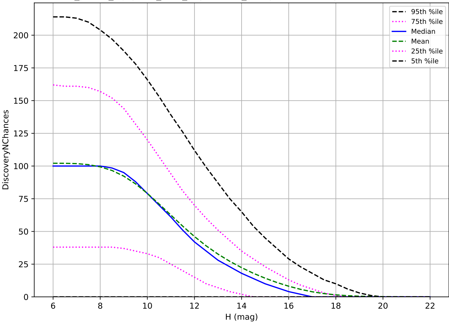
roll_pause_mjdp120_v3.4_10yrs: OCC_r5 3 pairs in 15 nights detection loss
