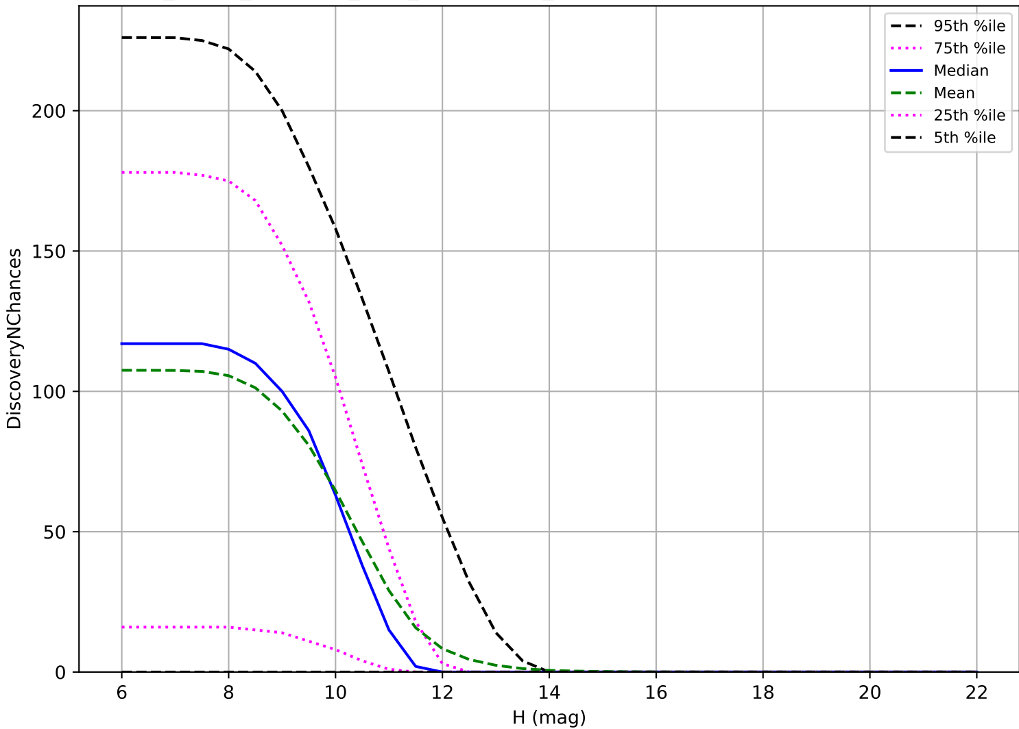
roll_pause_mjdp120_v3.4_10yrs: OCC_r20 3 pairs in 15 nights detection loss
