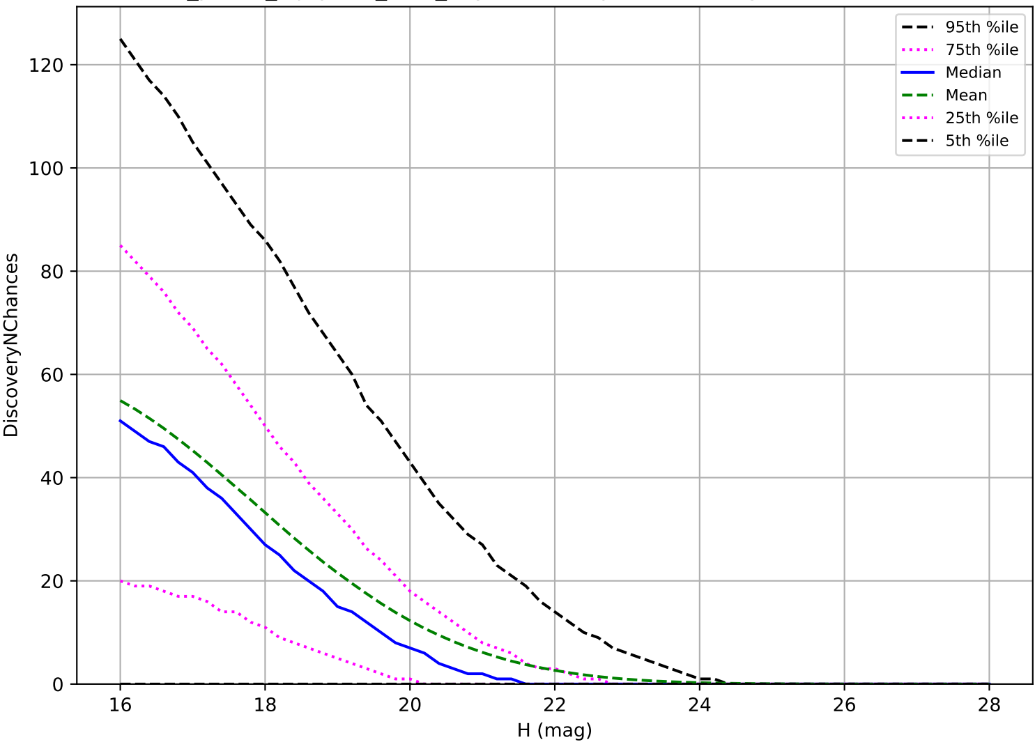
roll_pause_mjdp120_v3.4_10yrs: NEO 3 pairs in 15 nights detection loss
