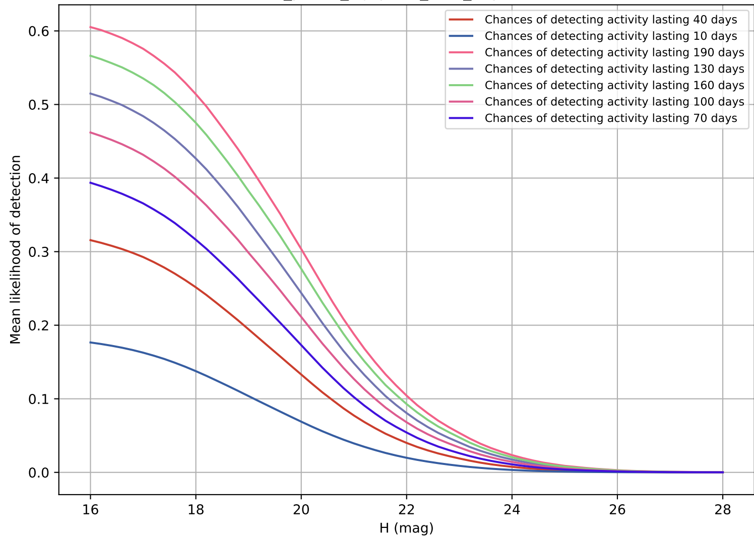
roll_pause_mjdp120_v3.4_10yrs PHA
