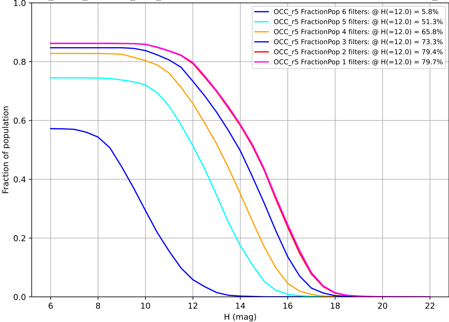
roll_pause_mjdp120_v3.4_10yrs: Fraction of population with colors in X filters OCC_r5
