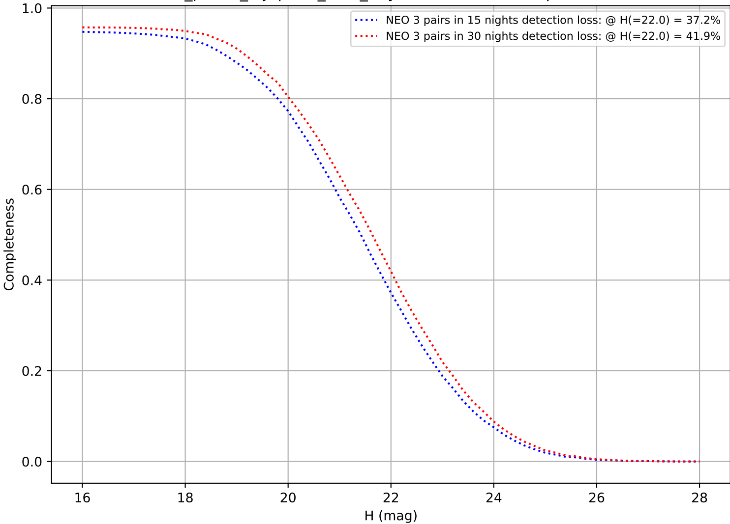
roll_pause_mjdp120_v3.4_10yrs: DifferentialCompleteness
