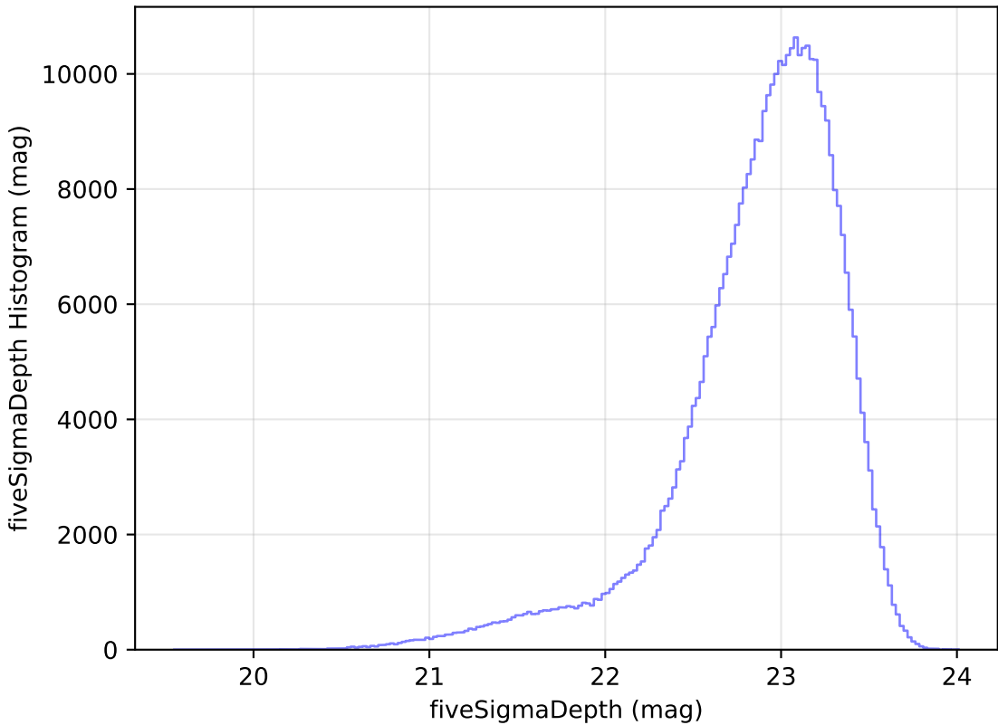
roll_pause_mjdp120_v3.4_10yrs z: fiveSigmaDepth Histogram
