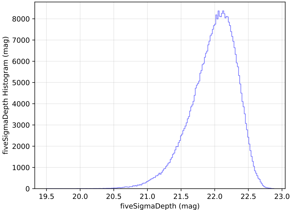
roll_pause_mjdp120_v3.4_10yrs y: fiveSigmaDepth Histogram
