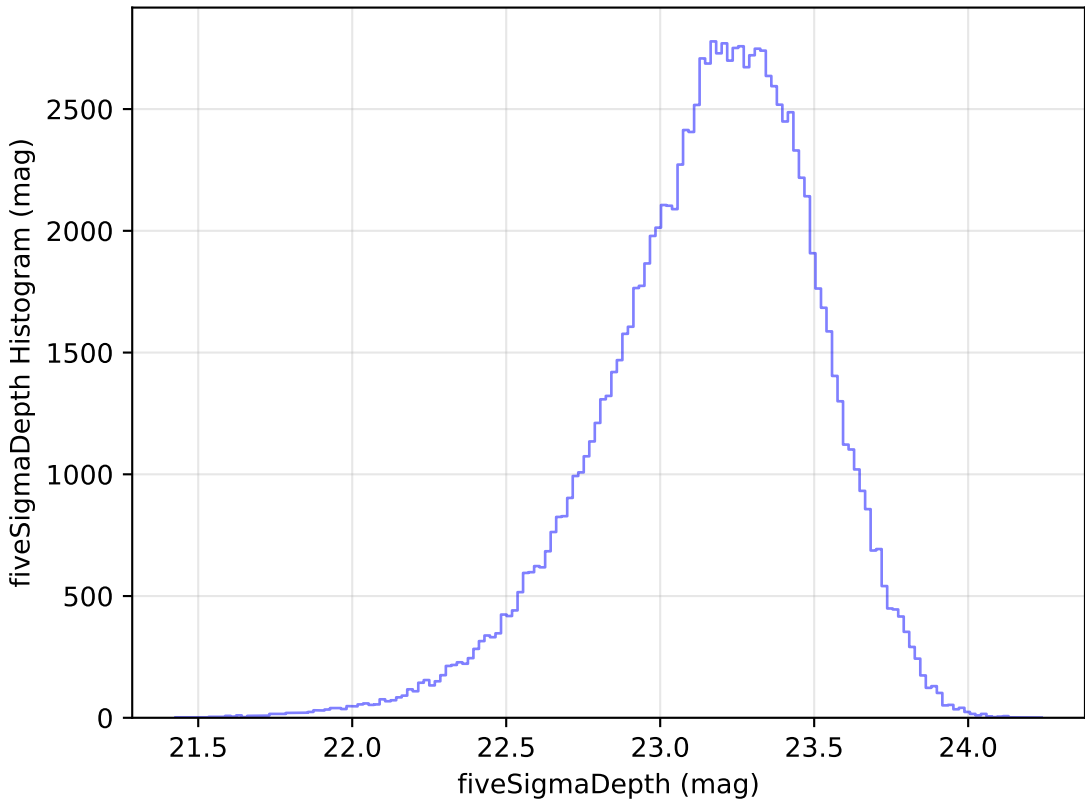
roll_pause_mjdp120_v3.4_10yrs u: fiveSigmaDepth Histogram
