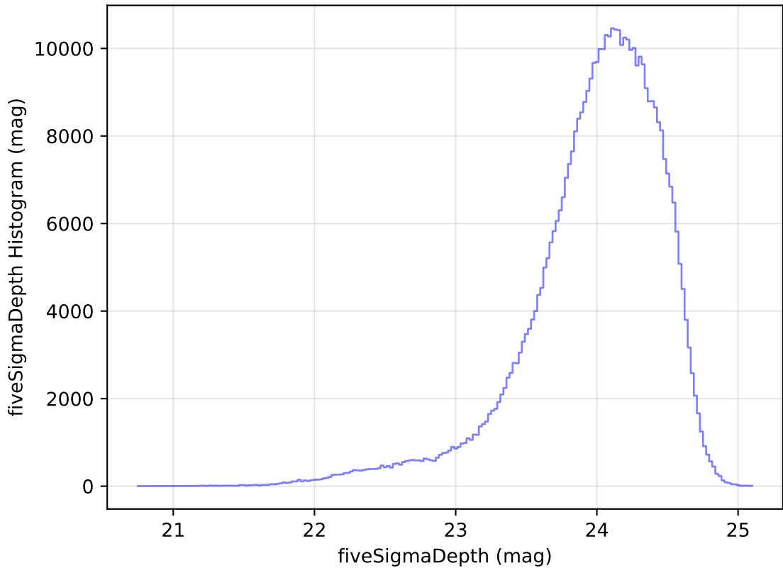
roll_pause_mjdp120_v3.4_10yrs r: fiveSigmaDepth Histogram
