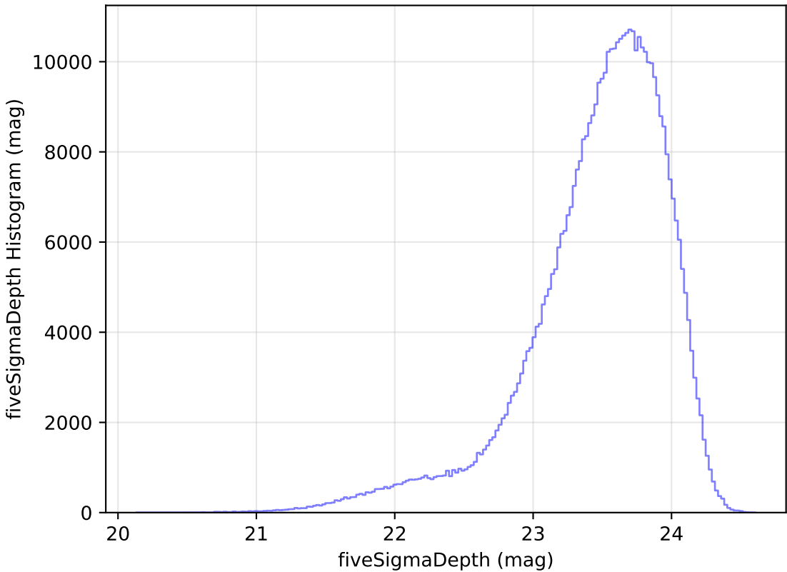
roll_pause_mjdp120_v3.4_10yrs i: fiveSigmaDepth Histogram
