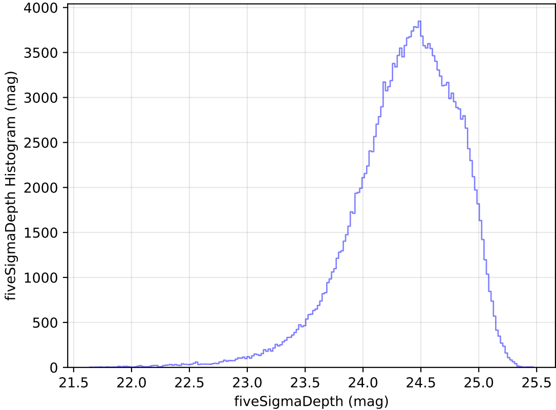
roll_pause_mjdp120_v3.4_10yrs g: fiveSigmaDepth Histogram
