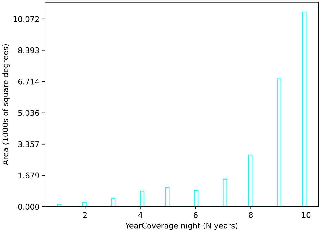
roll_pause_mjdp120_v3.4_10yrs u band: YearCoverage night
