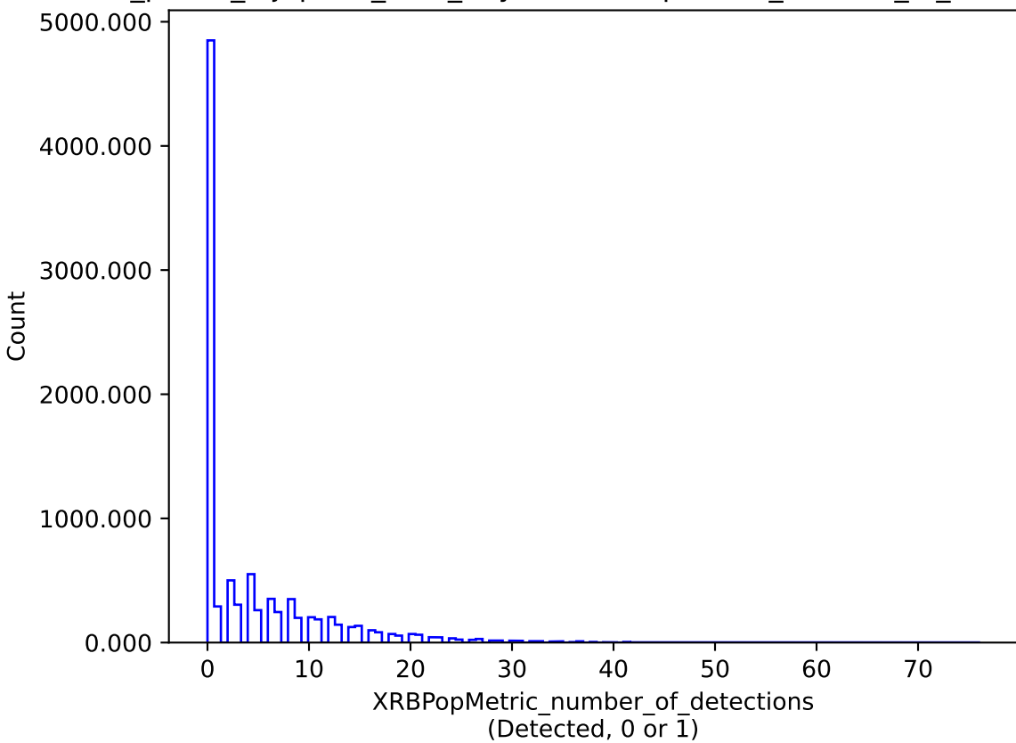
roll_pause_mjdp120_v3.4_10yrs : XRBPopMetric_number_of_detections
