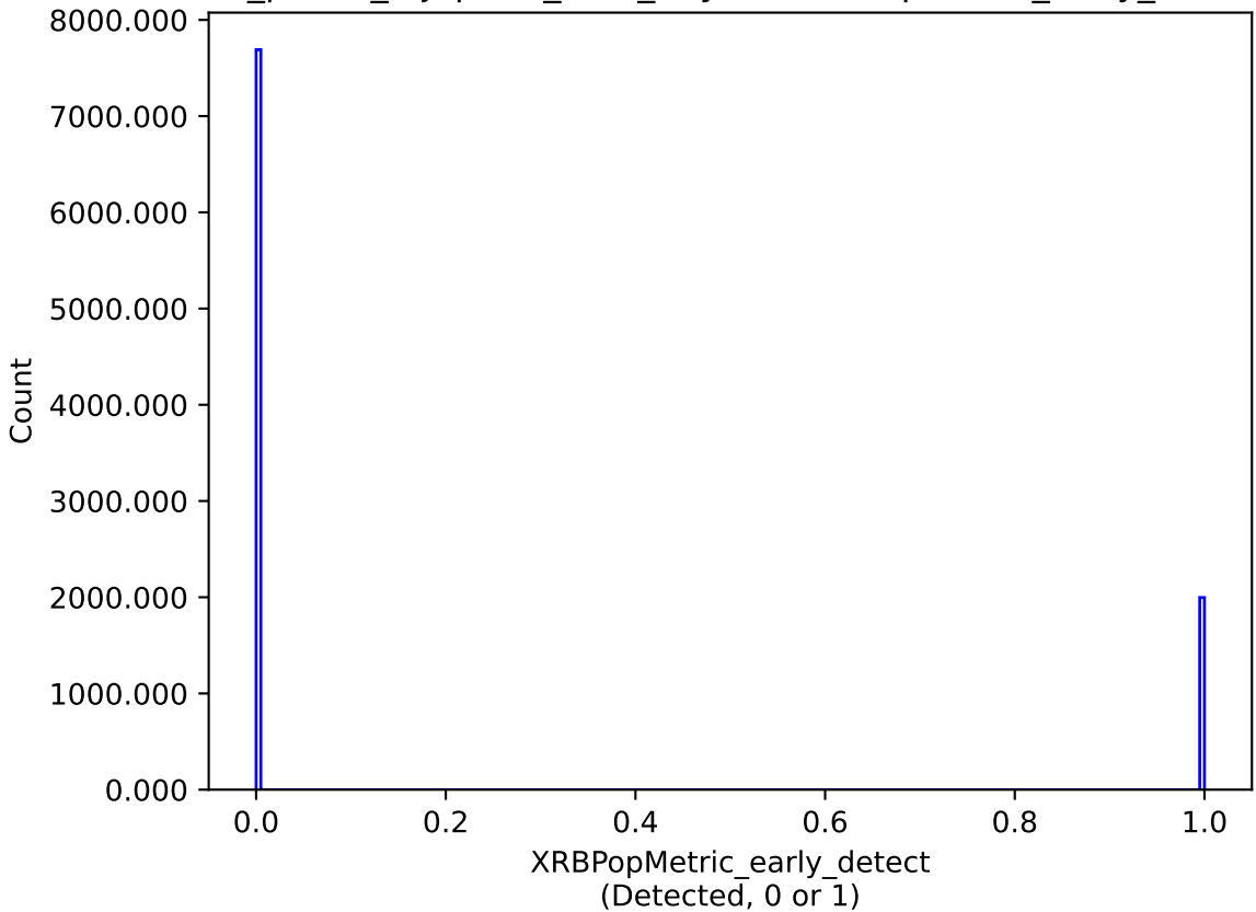
roll_pause_mjdp120_v3.4_10yrs : XRBPopMetric_early_detect
