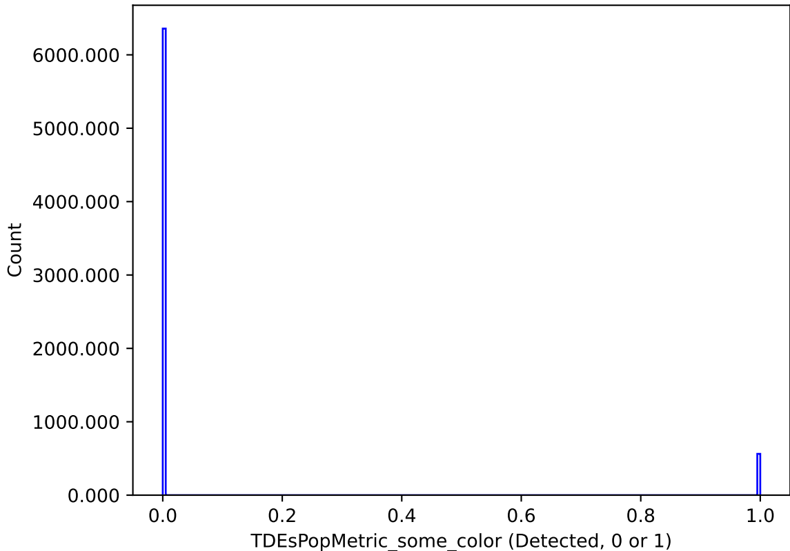
roll_pause_mjdp120_v3.4_10yrs : TDEsPopMetric_some_color
