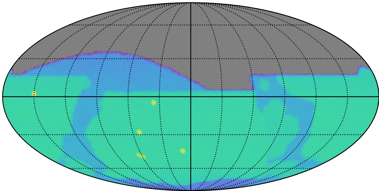
roll_pause_mjdp120_v3.4_10yrs z: SurfaceBrightLimit
