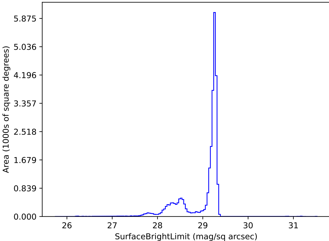
roll_pause_mjdp120_v3.4_10yrs z: SurfaceBrightLimit
