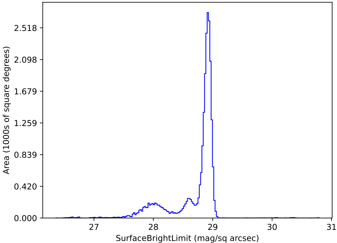
roll_pause_mjdp120_v3.4_10yrs u: SurfaceBrightLimit
