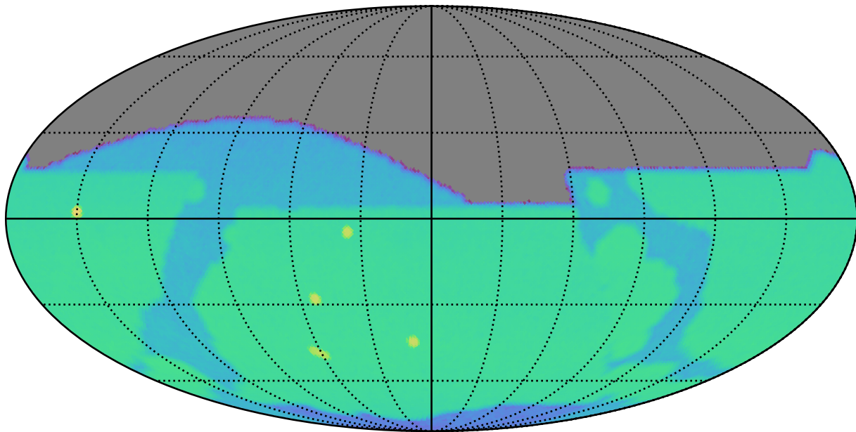
roll_pause_mjdp120_v3.4_10yrs r: SurfaceBrightLimit
