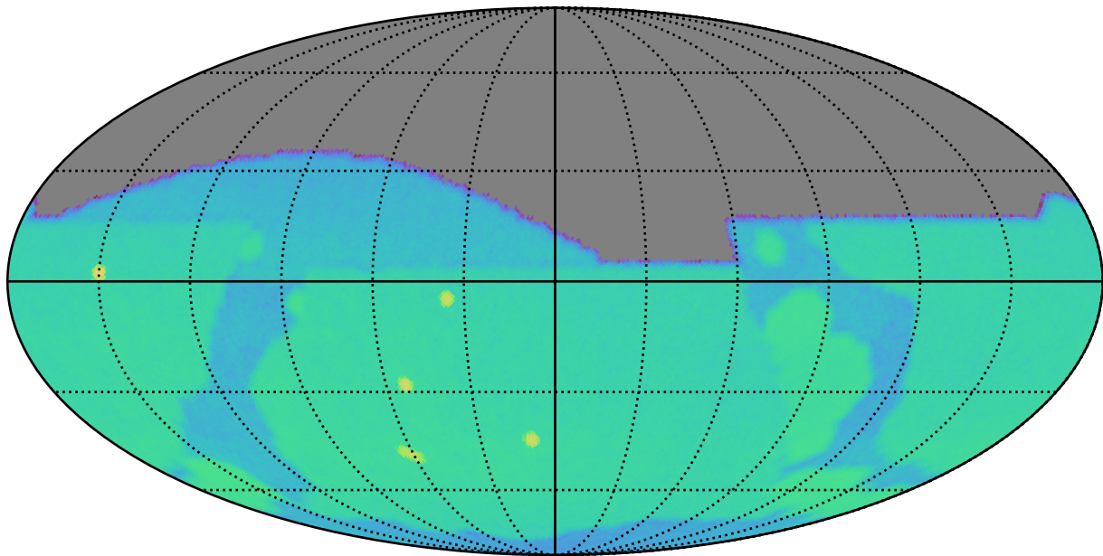
roll_pause_mjdp120_v3.4_10yrs g: SurfaceBrightLimit
