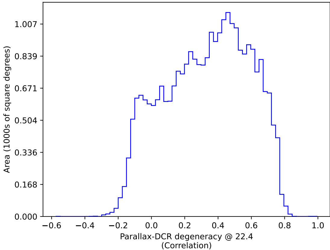
roll_pause_mjdp120_v3.4_10yrs : Parallax-DCR degeneracy @ 22.4
