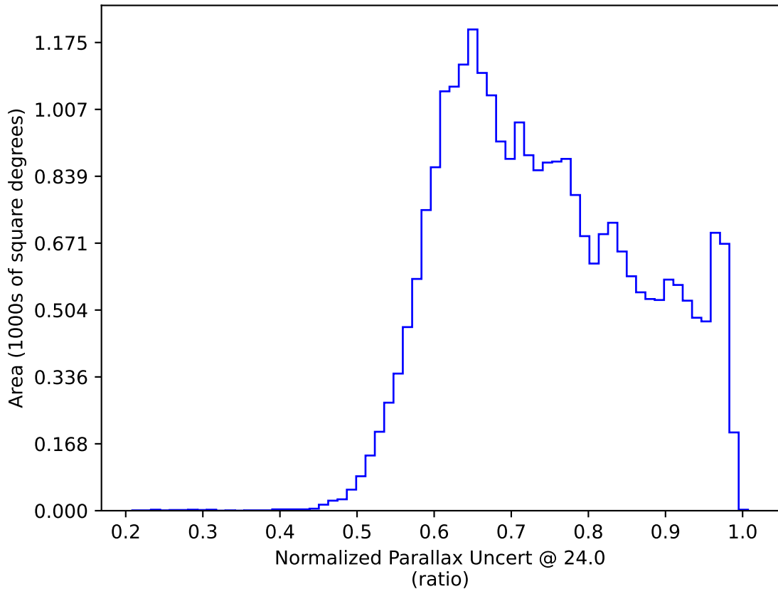
roll_pause_mjdp120_v3.4_10yrs : Normalized Parallax Uncert @ 24.0
