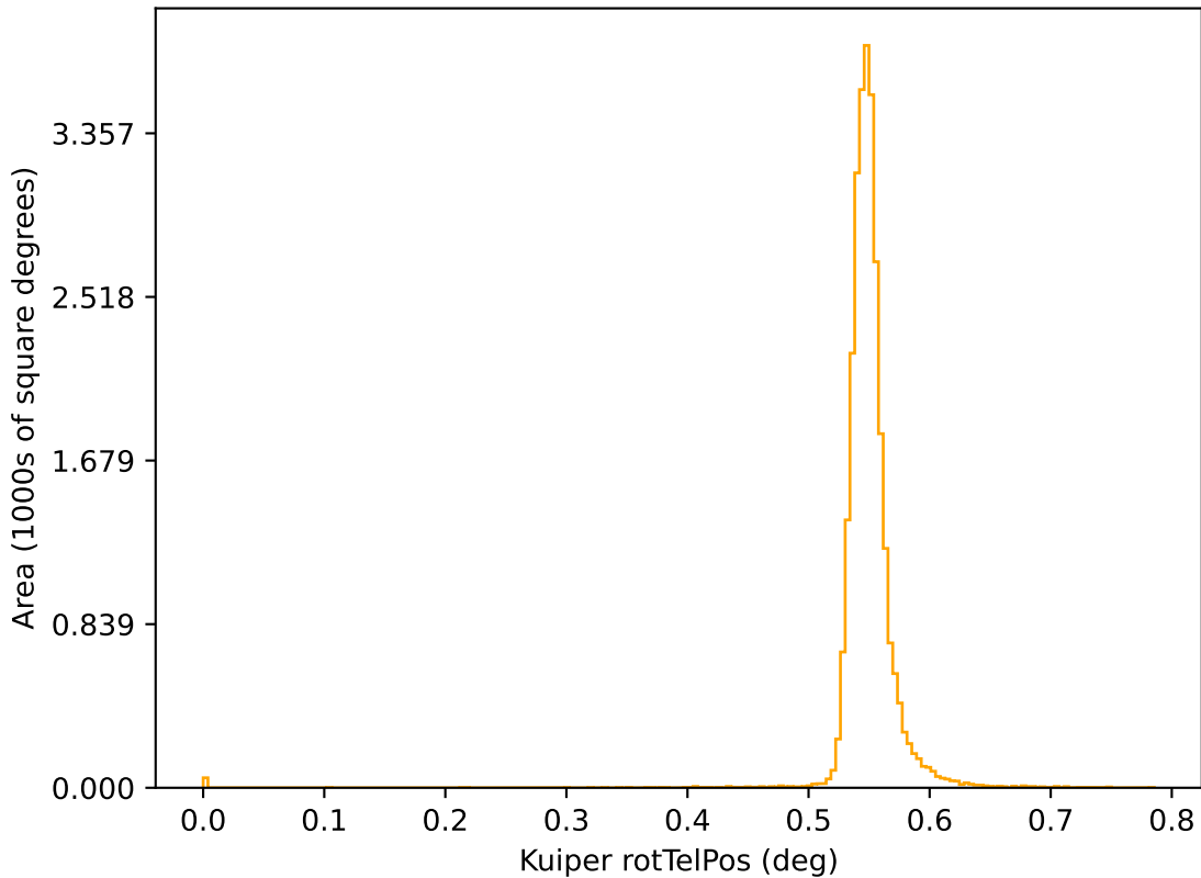
roll_pause_mjdp120_v3.4_10yrs r: Kuiper rotTelPos
