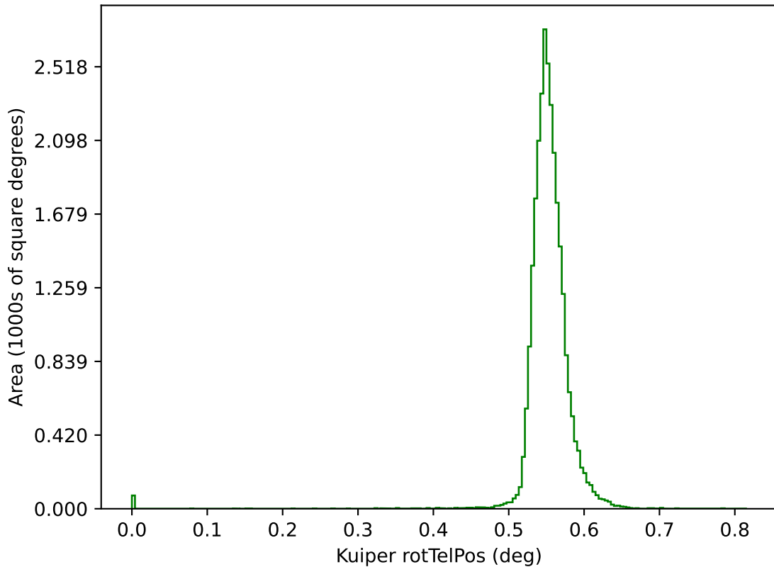
roll_pause_mjdp120_v3.4_10yrs g: Kuiper rotTelPos
